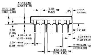
Order Number MM74HC30N NS Package N14A
