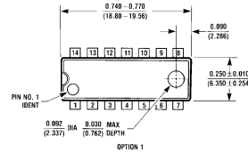
Order Number MM54HC30J or MM74HC30J NS Package J14A
